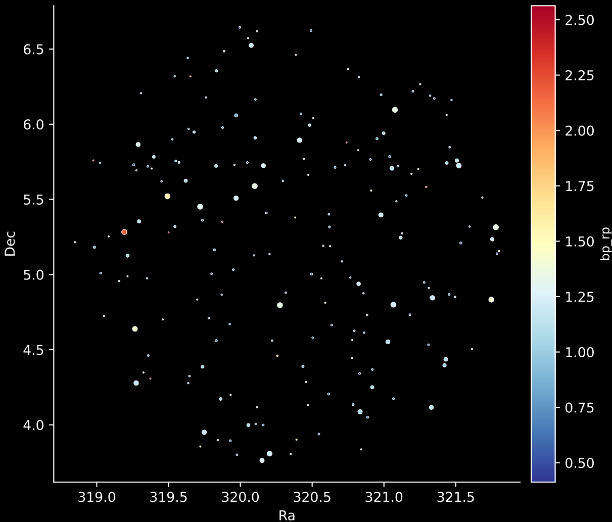
APOGEE DR17 Field: [358+56_MGA] Stars: 187
