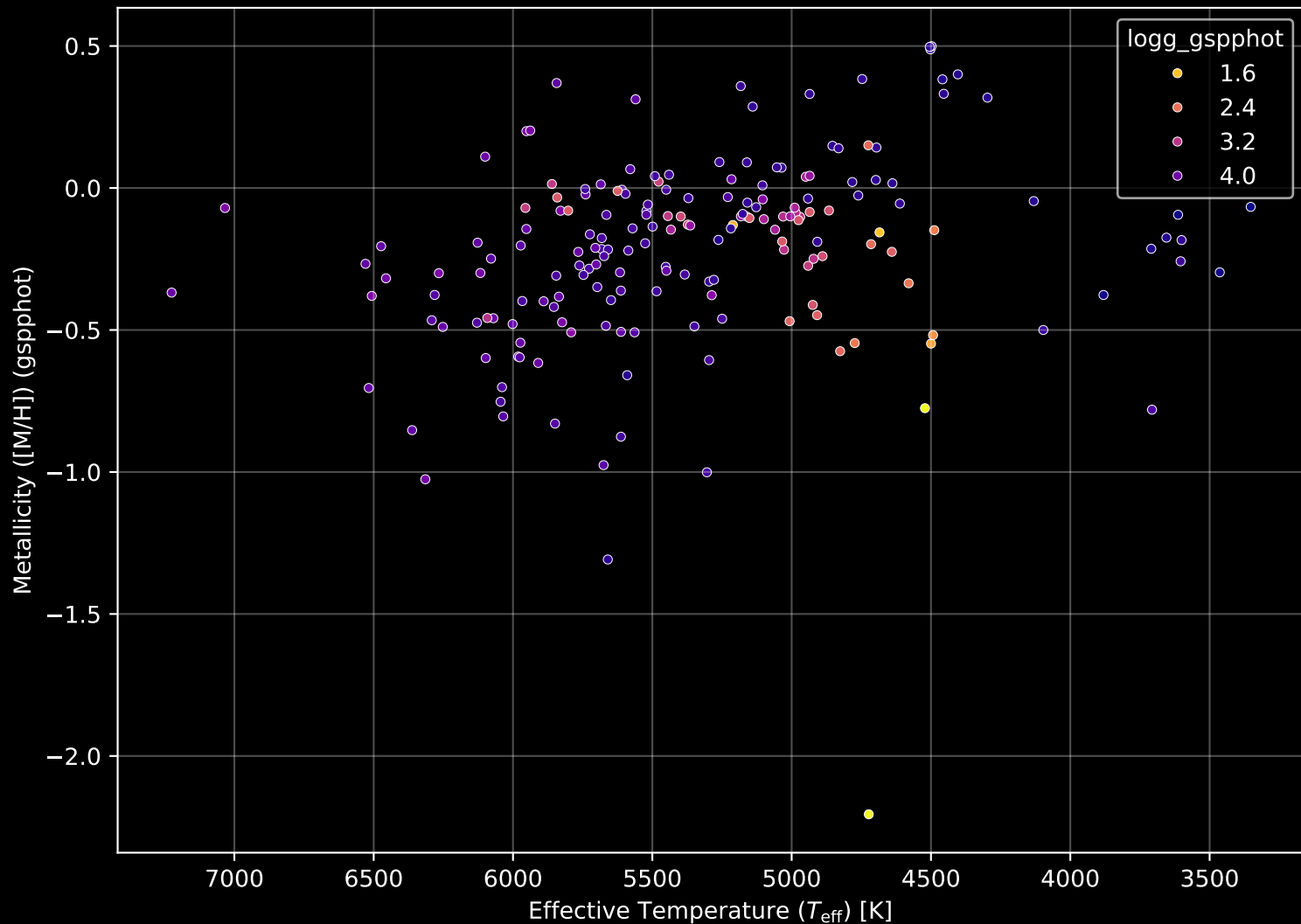
APOGEE DR17 Field: [358+56_MGA] Stellar Population Parameters (n= 187)
