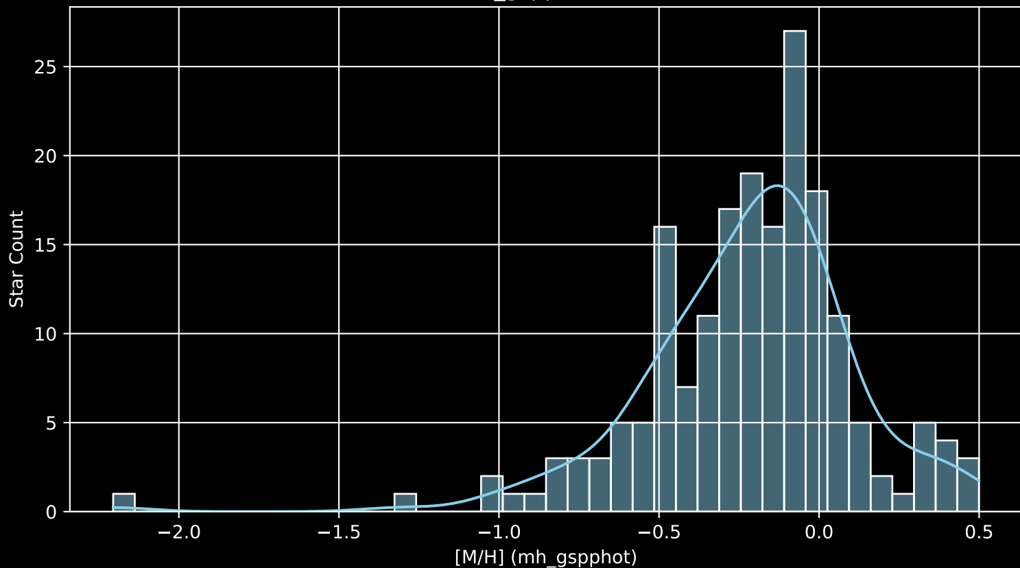
APOGEE DR17 Field: [358+56_MGA [M/H] (mh_gspphot) (n= 187)
