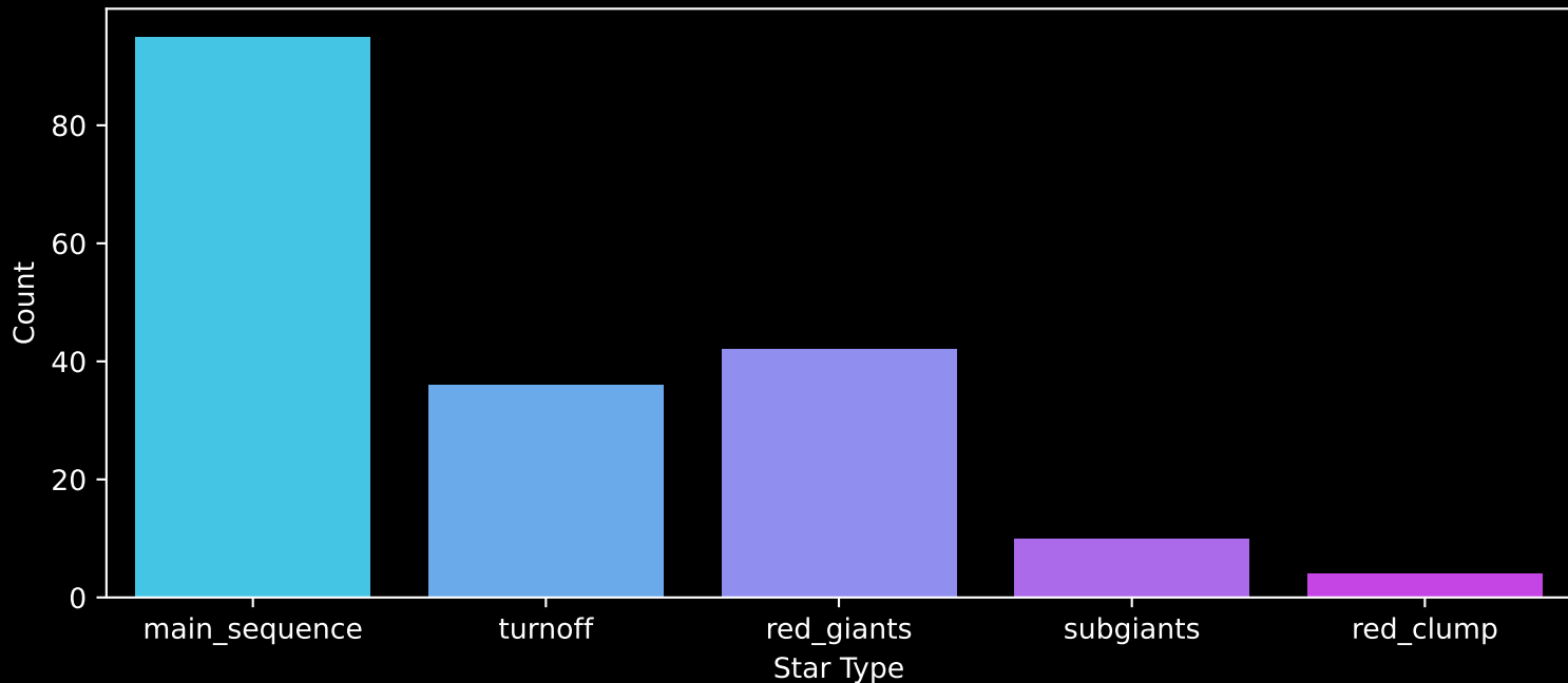
APOGEE DR17 Field: [358+56_MGA] Count plot of Star Type
