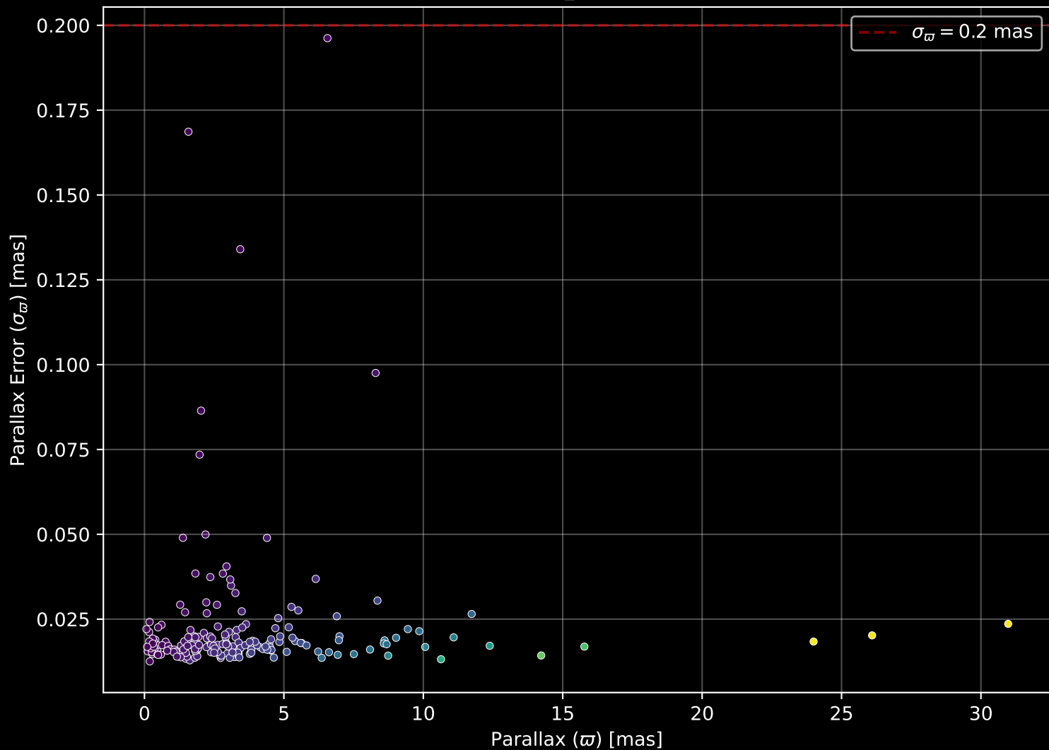
APOGEE DR17 Field: [358+56_MGA] Parallax Quality (n= 187)
