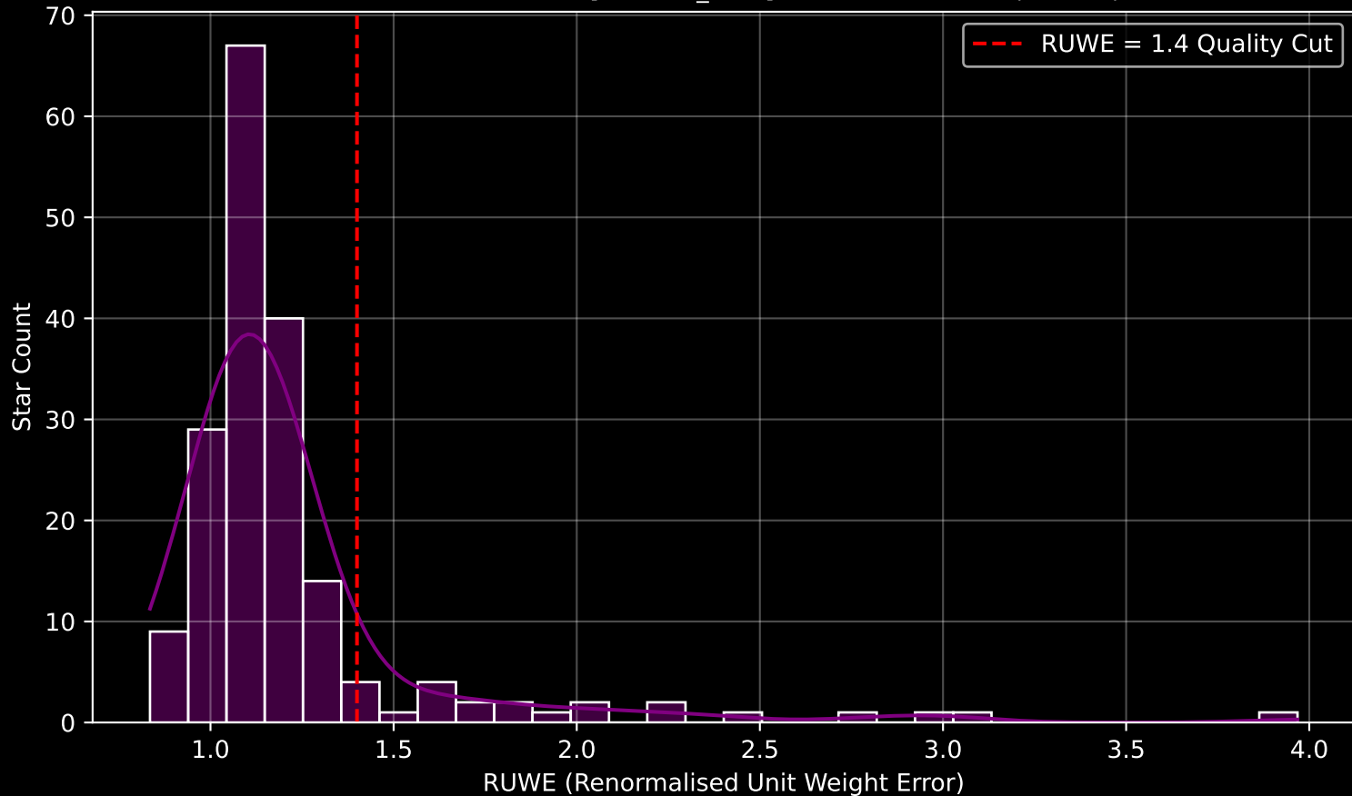
GAPOGEE DR17 Field [358+56_MGA] RUWE Distribution (n= 182)
