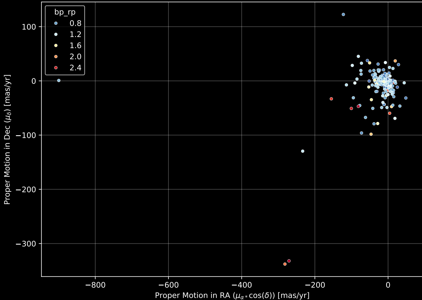
APOGEE DR17 Field: [358+56_MGA] Proper Motion Diagram (n= 187)
